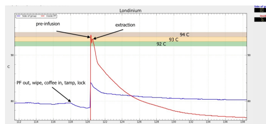
Figure 9. Extraction temperature profile
